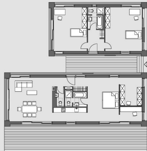
kids house extension 1:250
