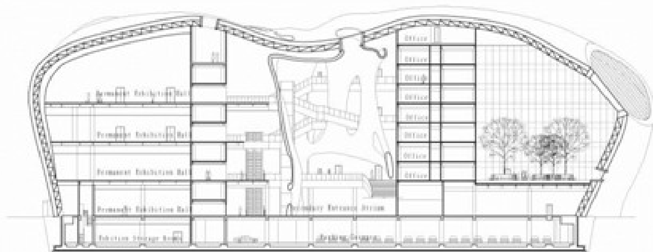
Section 2-2
