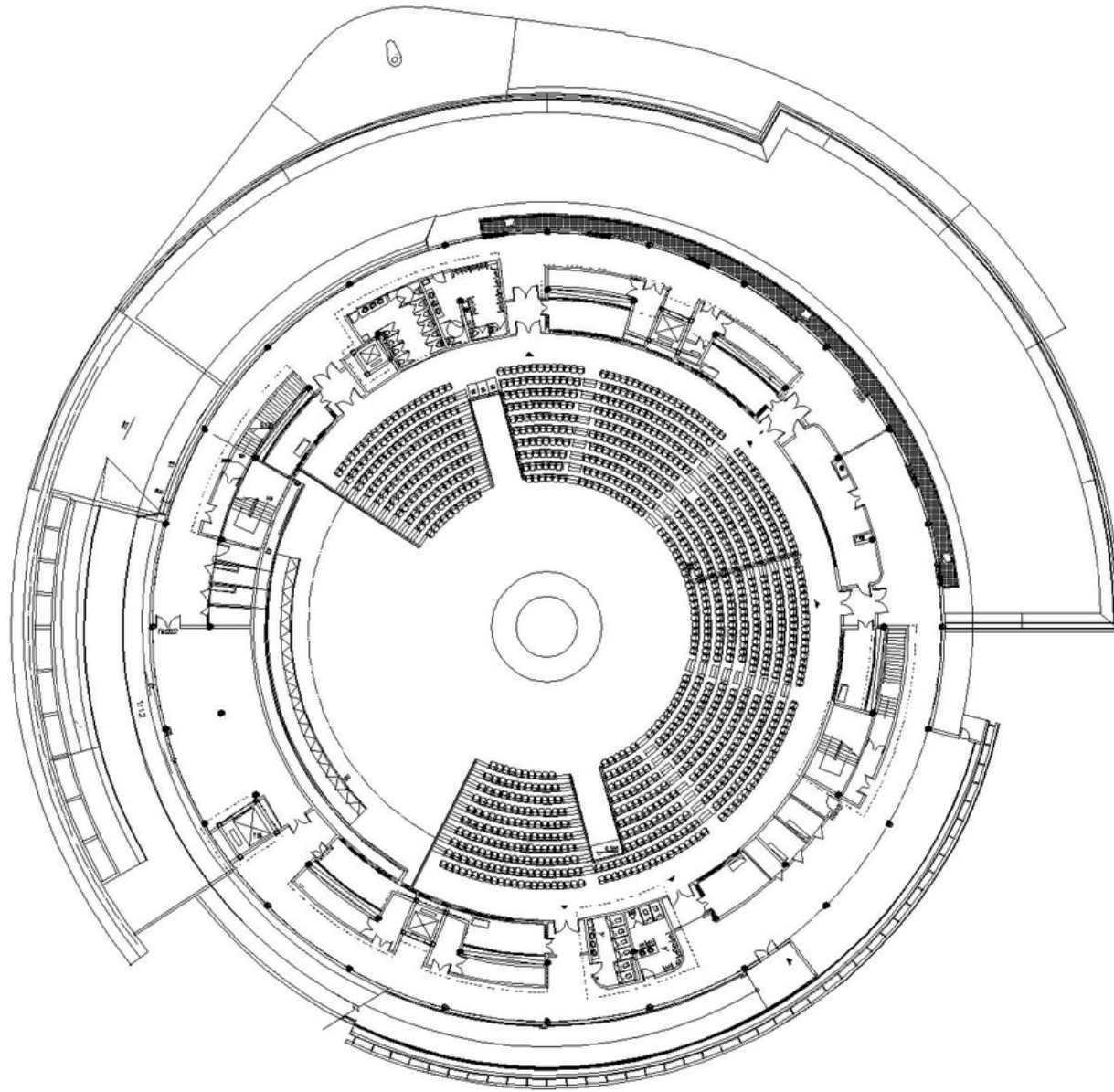
SAIC - GM FIRST FLOOR PLAN 1:100
