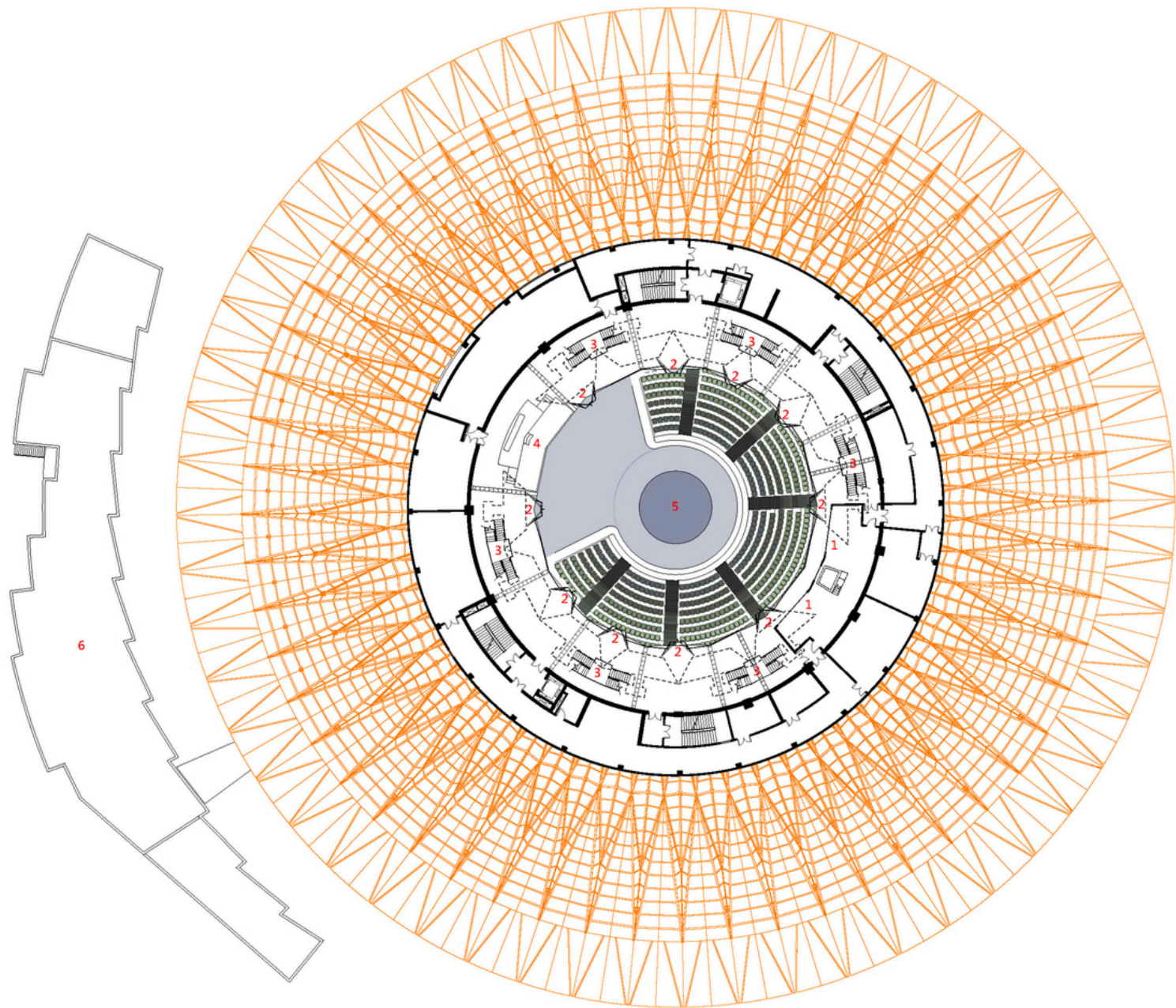
CONTROL PLAN +9.00m
